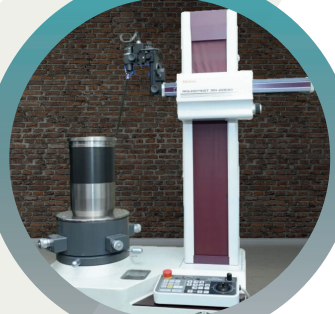
Roundness Tester
